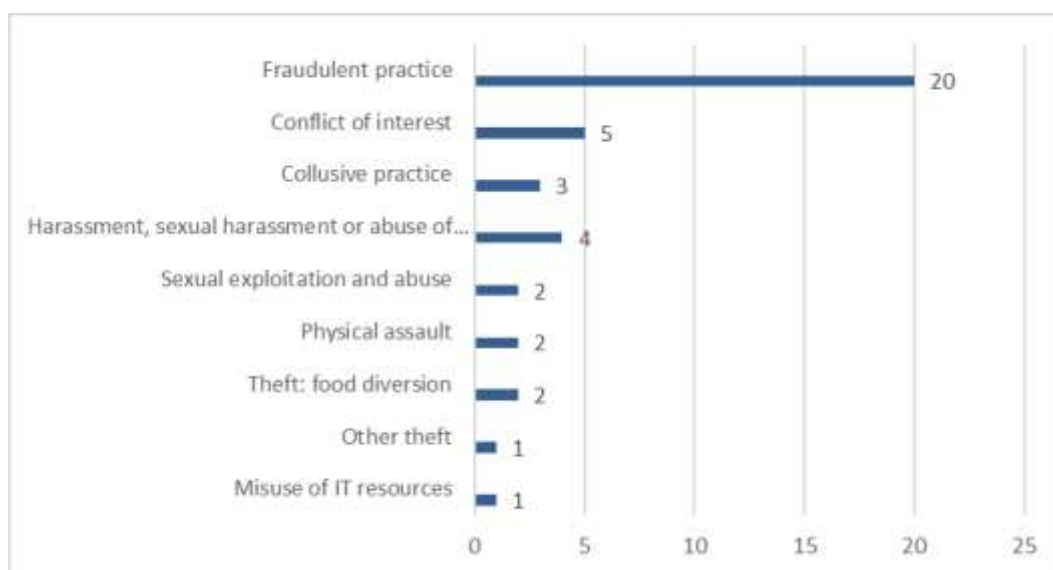
Figure 1: Investigations Completed, by Case Type in 2017
