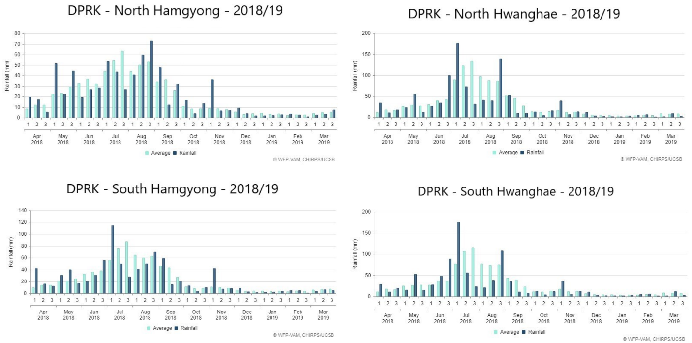
FIGURE 3: DPRK - RAINFALL AMOUNTS (RFE) FROM APRIL 2018-MARCH 2019
